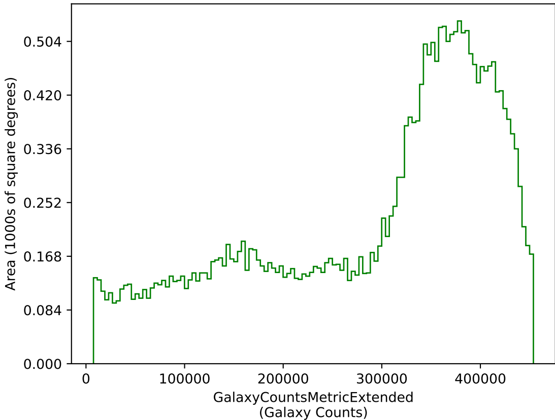
extra_ss_neo4_v3.4_10yrs g: GalaxyCountsMetricExtended
