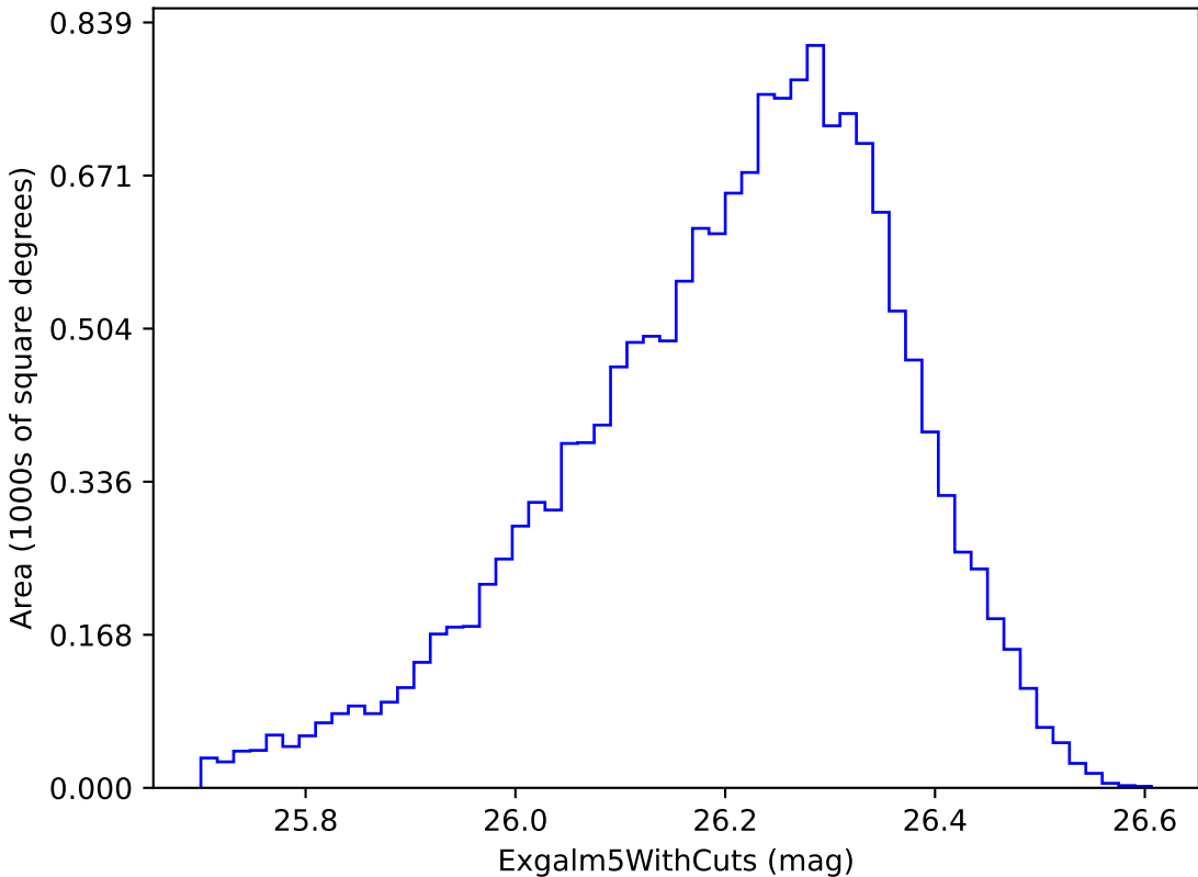
extra_ss_neo4_v3.4_10yrs i band non-DD year 7: ExgalM5WithCuts
