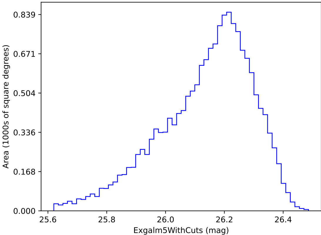
extra_ss_neo4_v3.4_10yrs i band non-DD year 6: ExgalM5WithCuts
