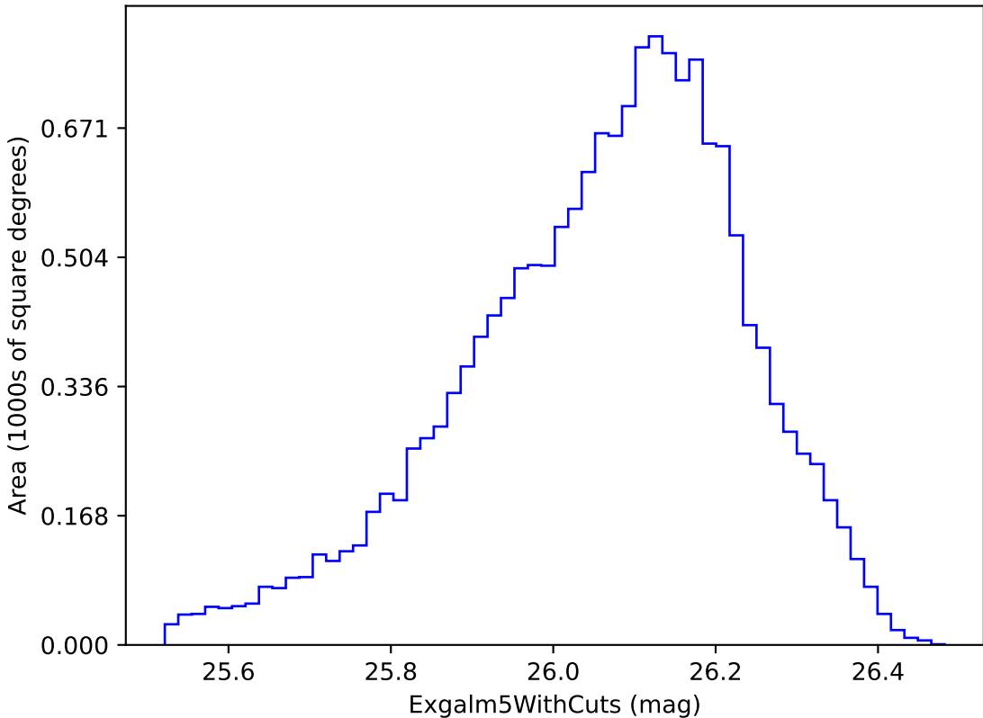
extra_ss_neo4_v3.4_10yrs i band non-DD year 5: ExgalM5WithCuts
