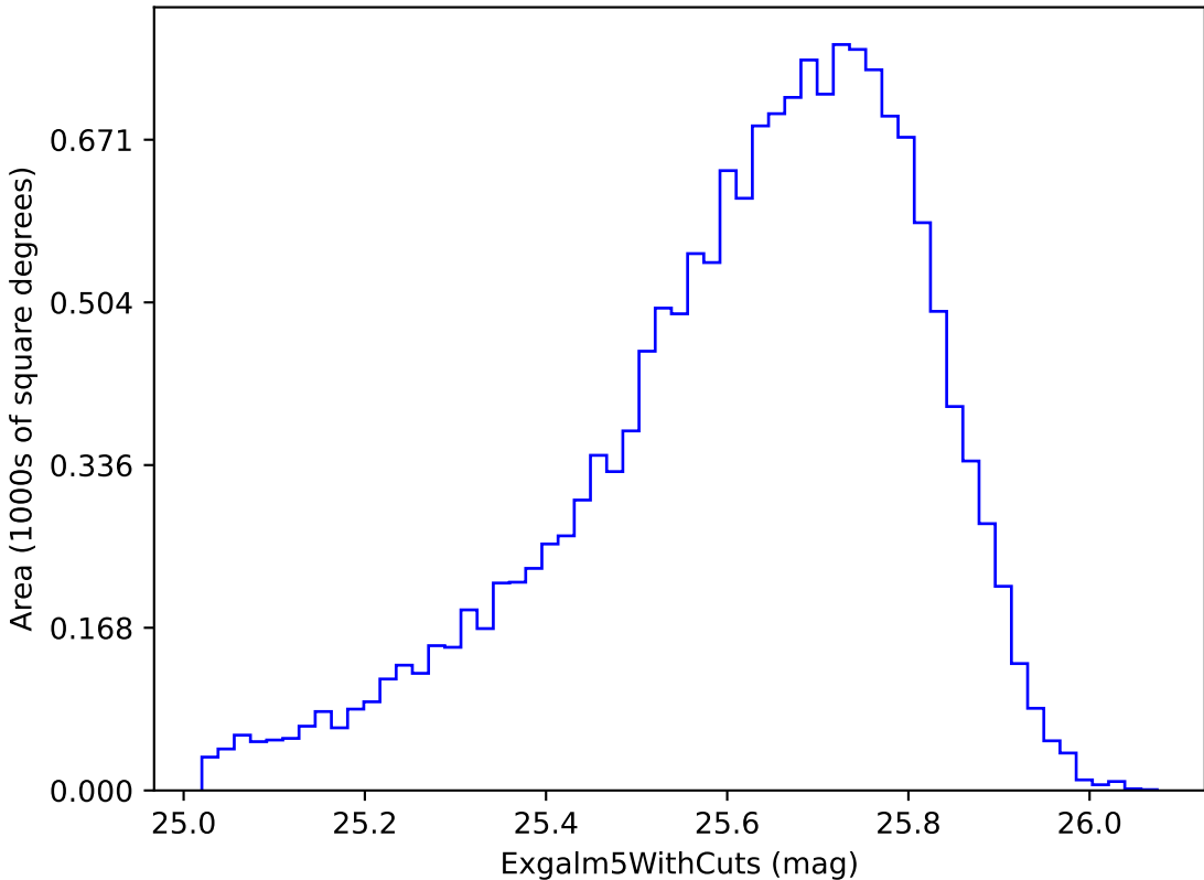
extra_ss_neo4_v3.4_10yrs i band non-DD year 2: ExgalM5WithCuts
