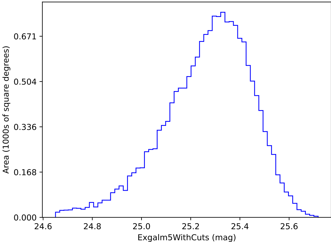
extra_ss_neo4_v3.4_10yrs i band non-DD year 1: Exgalml5WithCuts
