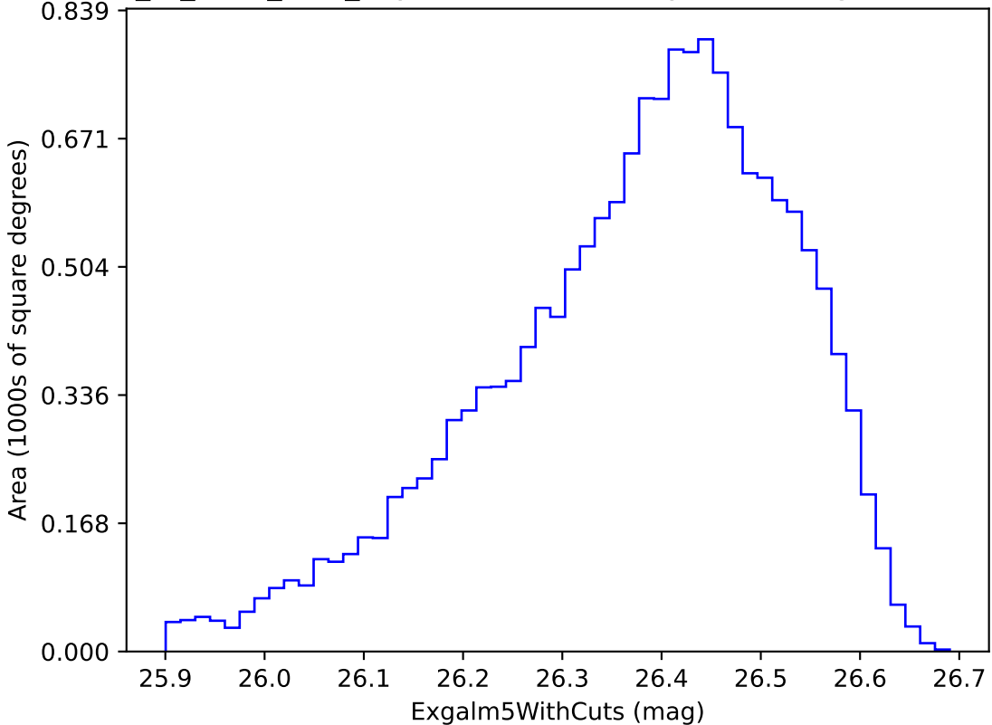
extra_ss_neo4_v3.4_10yrs i band non-DD year 10: ExgalM5WithCuts
