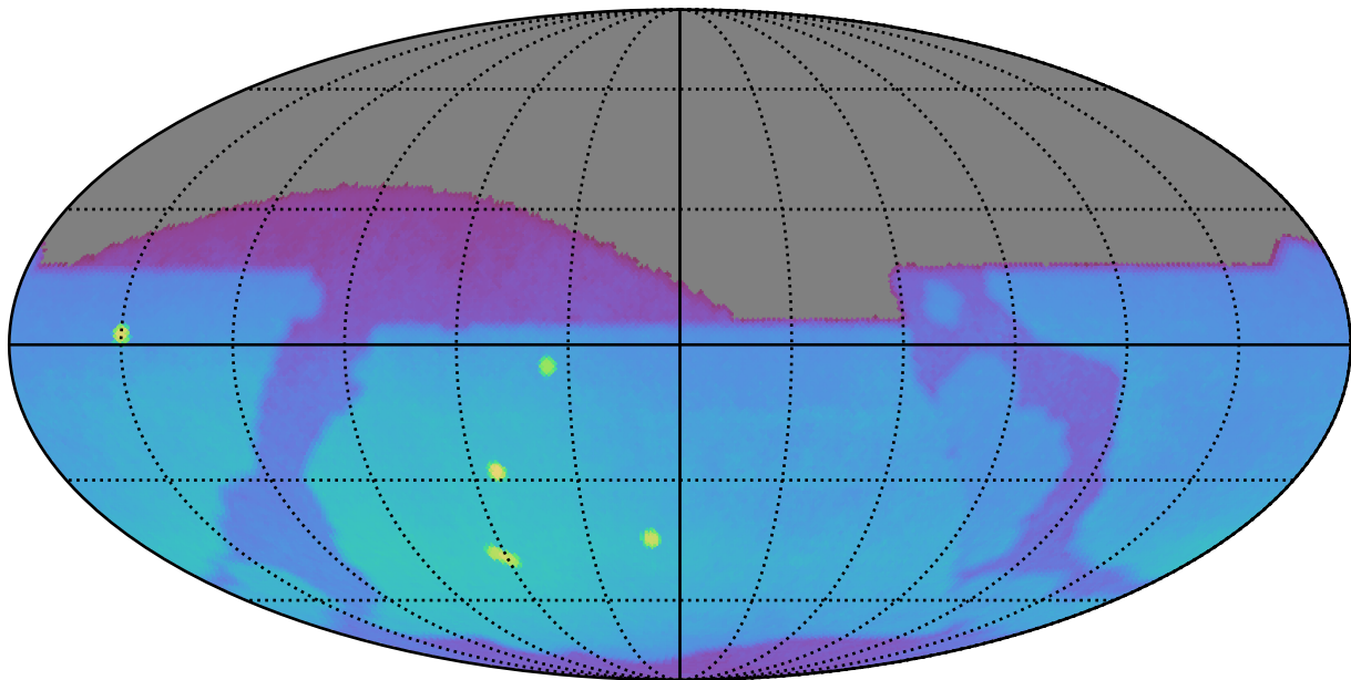
extra_ss_neo4_v3.4_10yrs : Brown Dwarf, L7
