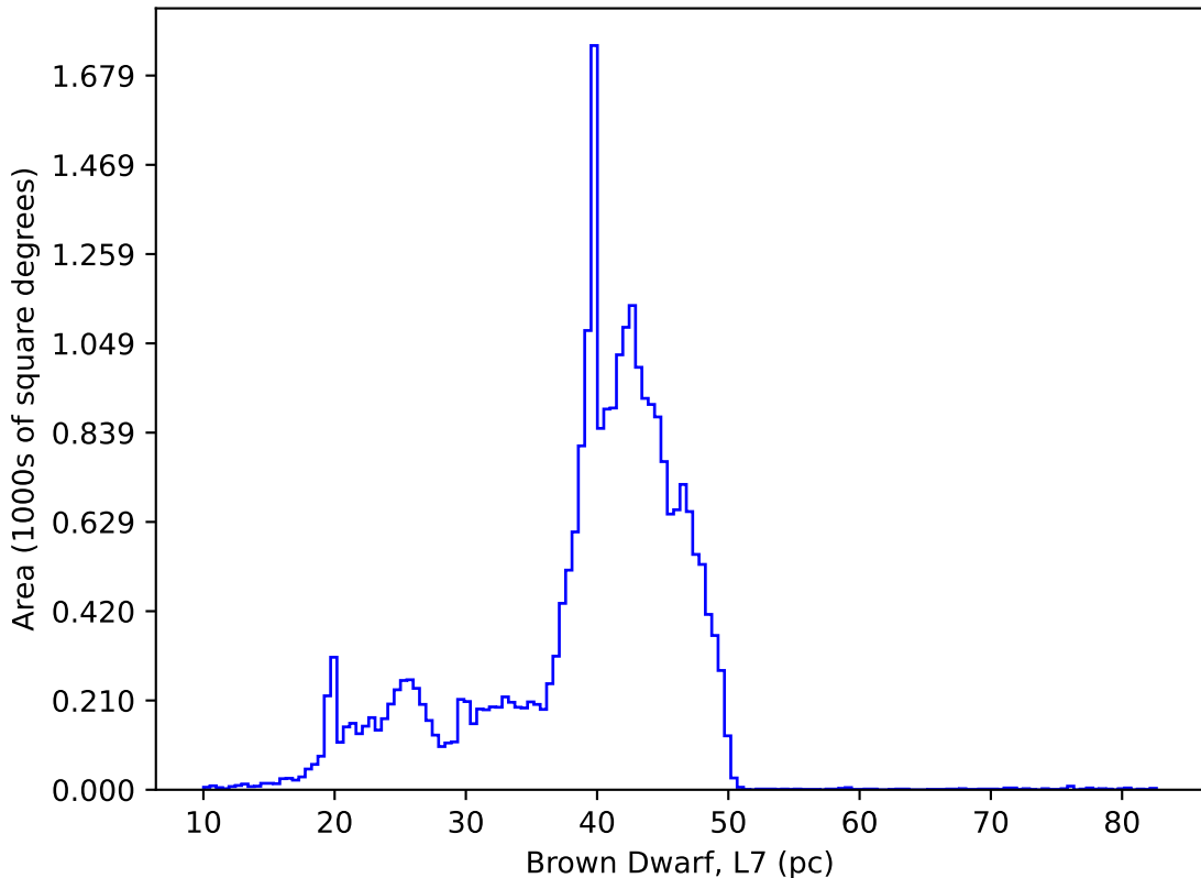
extra_ss_neo4_v3.4_10yrs : Brown Dwarf, L7
