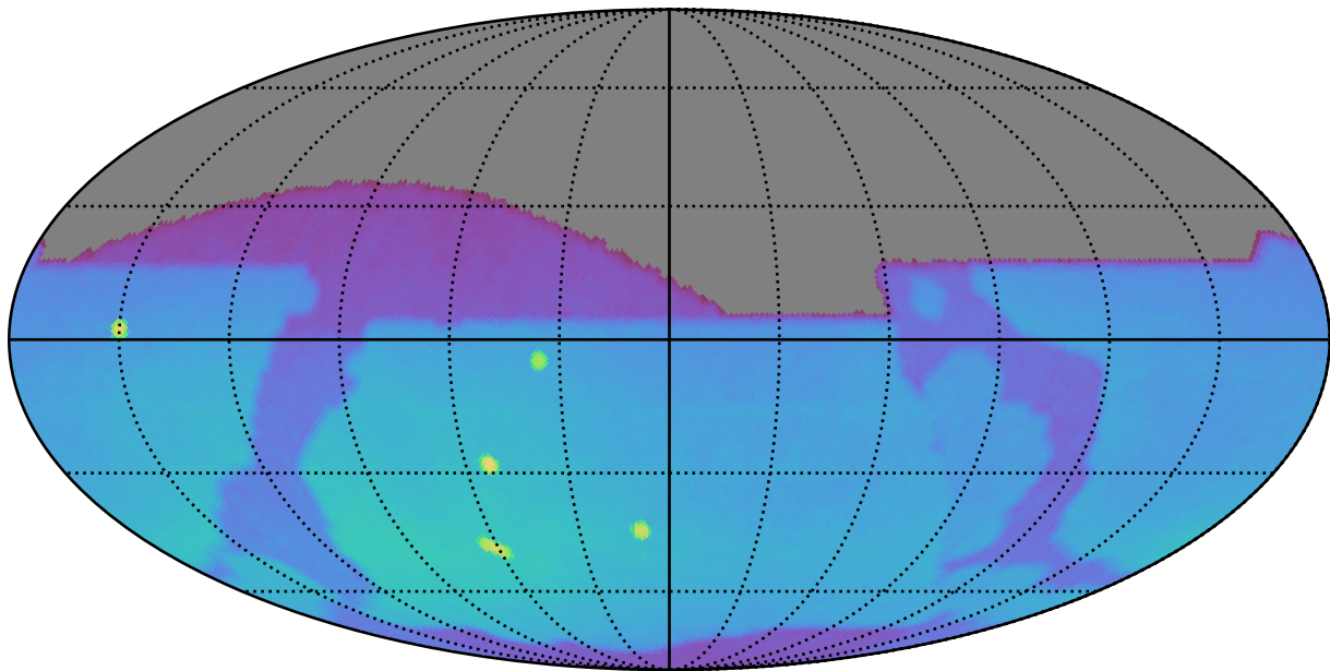
extra_ss_neo4_v3.4_10yrs : Brown Dwarf, L4
