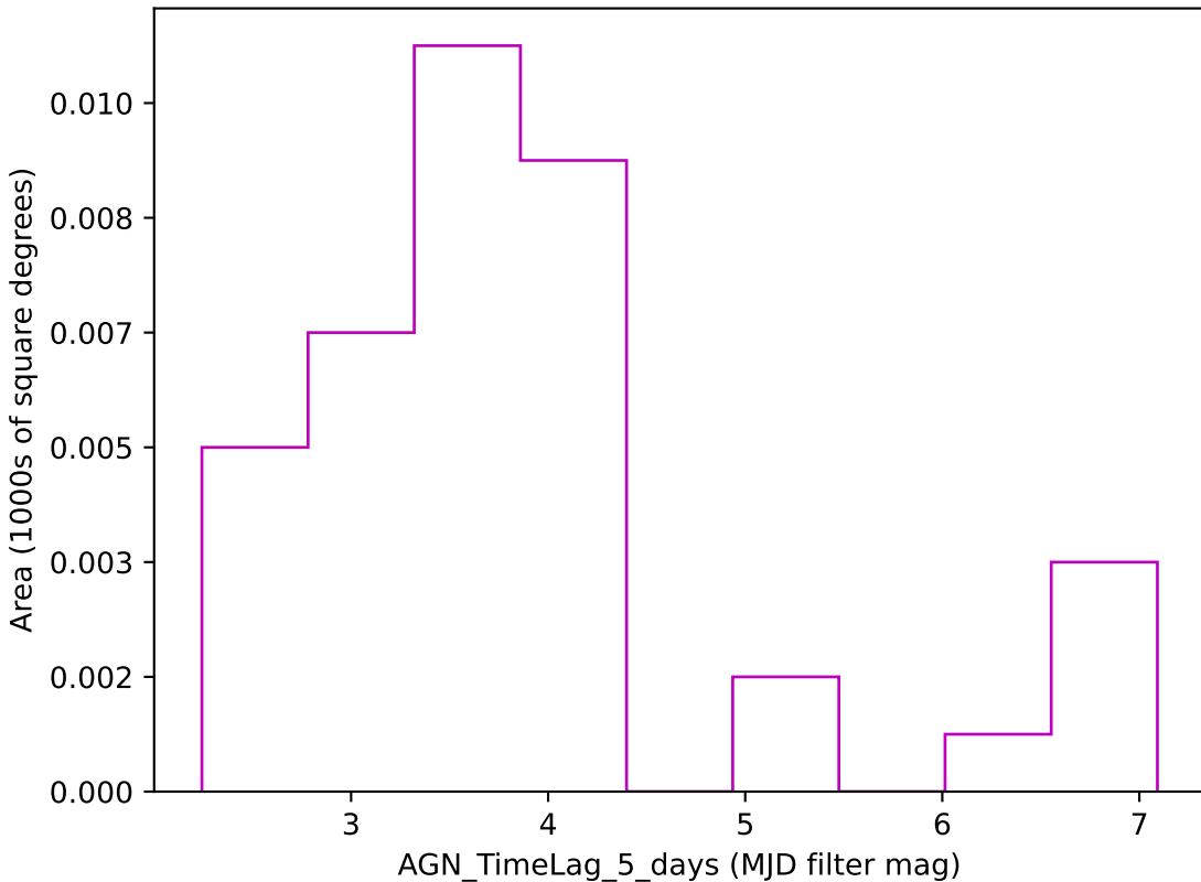
extra_ss_neo4_v3.4_10yrs z band: AGN_TimeLag_5_days
