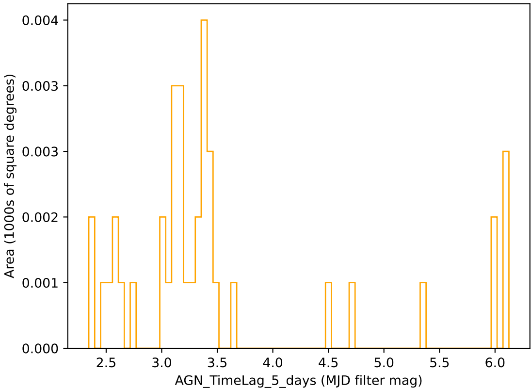
extra_ss_neo4_v3.4_10yrs r band: AGN_TimeLag_5_days
