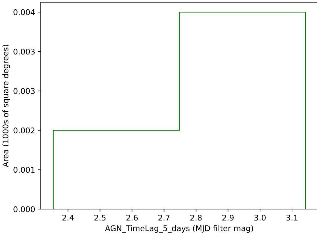
extra_ss_neo4_v3.4_10yrs g band: AGN_TimeLag_5_days
