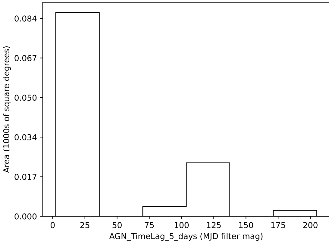
extra_ss_neo4_v3.4_10yrs all bands: AGN_TimeLag_5_days
