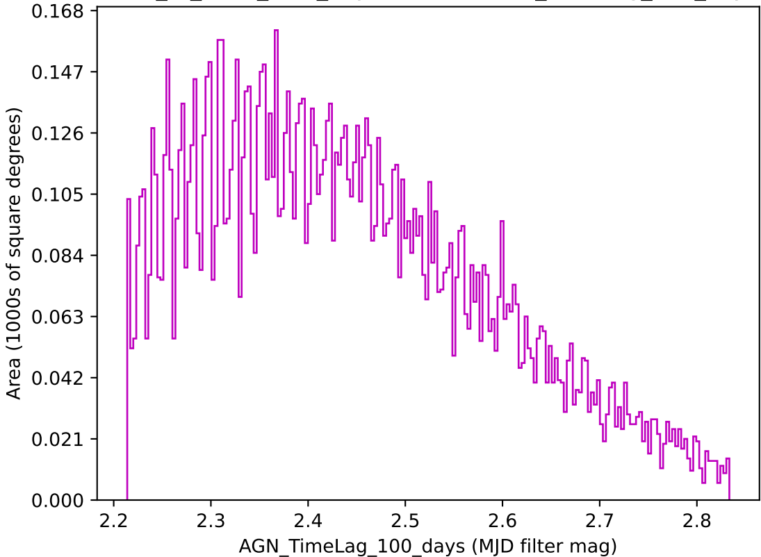
extra_ss_neo4_v3.4_10yrs z band: AGN_TimeLag_100_days
