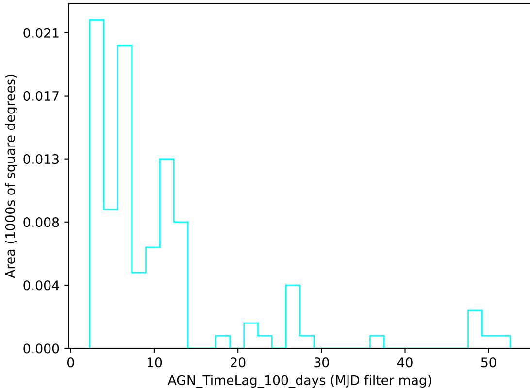
extra_ss_neo4_v3.4_10yrs u band: AGN_TimeLag_100_days
