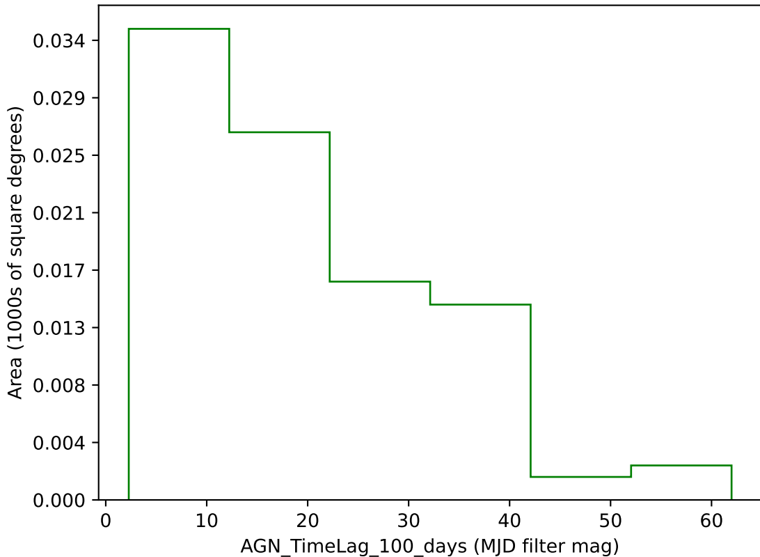
extra_ss_neo4_v3.4_10yrs g band: AGN_TimeLag_100_days
