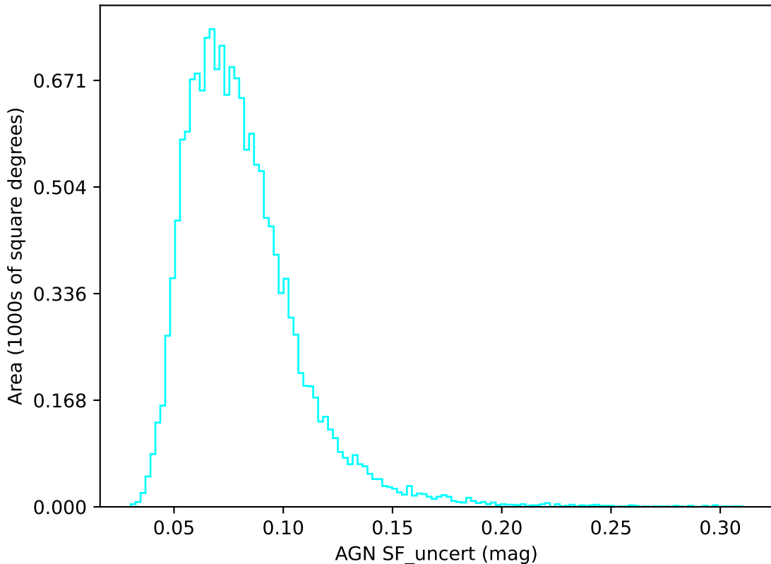
extra_ss_neo4_v3.4_10yrs u band: AGN SF_uncert
