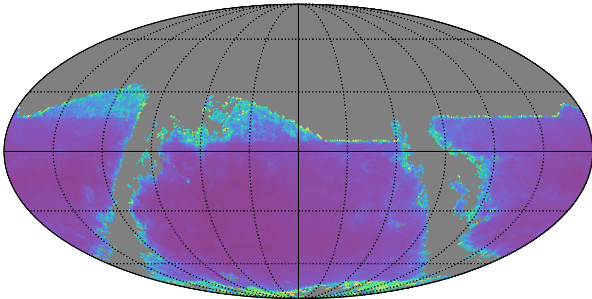
extra_ss_neo4_v3.4_10yrs r band: AGN SF_uncert
