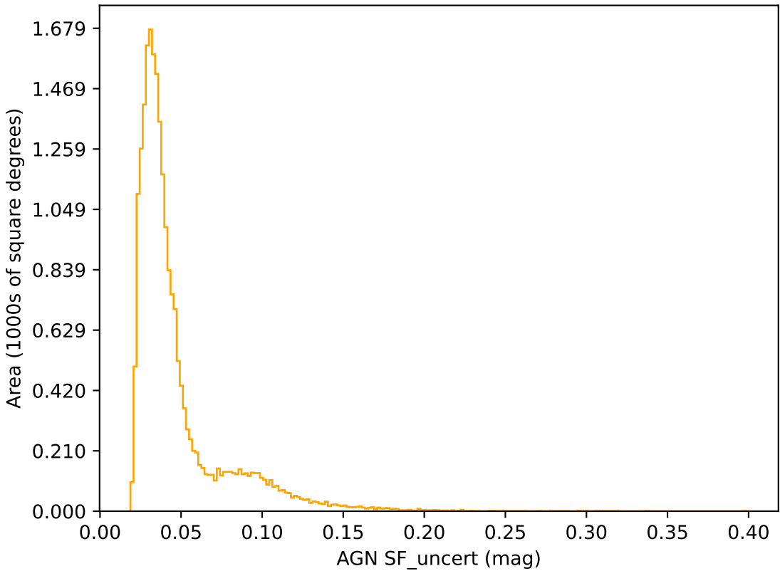
extra_ss_neo4_v3.4_10yrs r band: AGN SF_uncert
