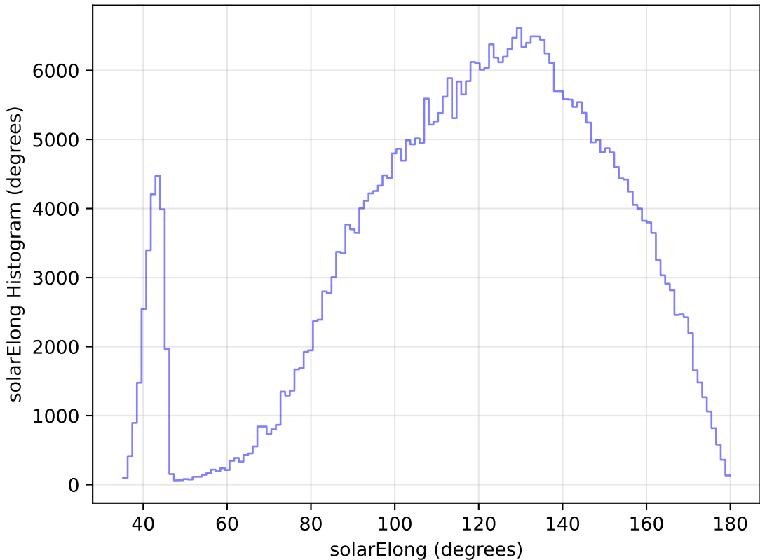
extra_ss_neo4_v3.4_10yrs WFD z band: solarElong Histogram
