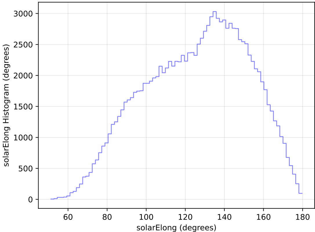
extra_ss_neo4_v3.4_10yrs WFD u band: solarElong Histogram
