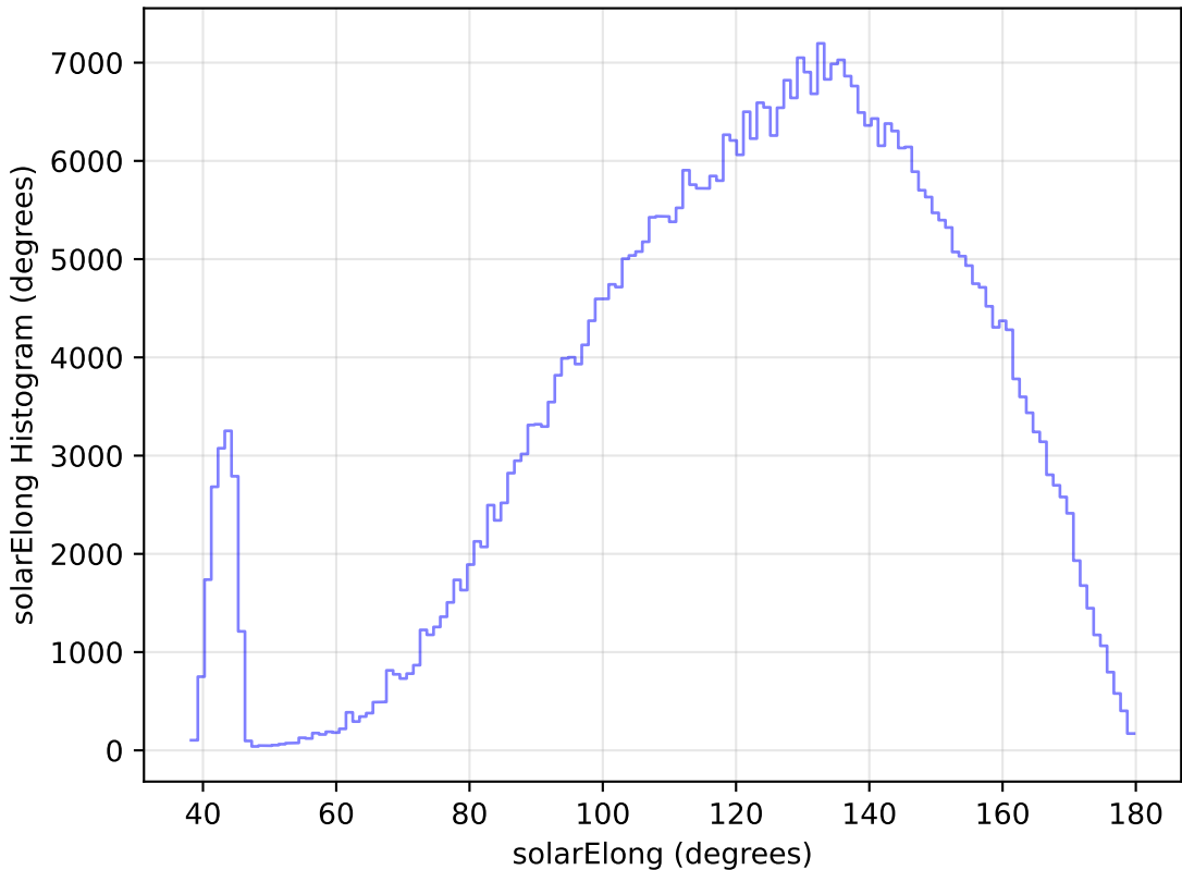
extra_ss_neo4_v3.4_10yrs WFD r band: solarElong Histogram
