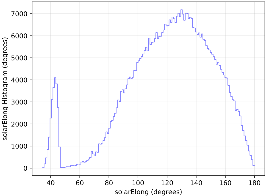
extra_ss_neo4_v3.4_10yrs WFD i band: solarElong Histogram
