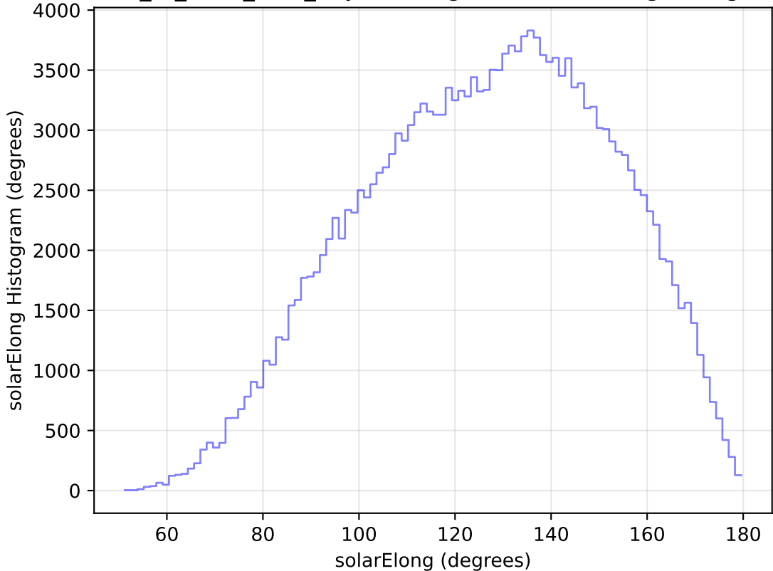
extra_ss_neo4_v3.4_10yrs WFD g band: solarElong Histogram
