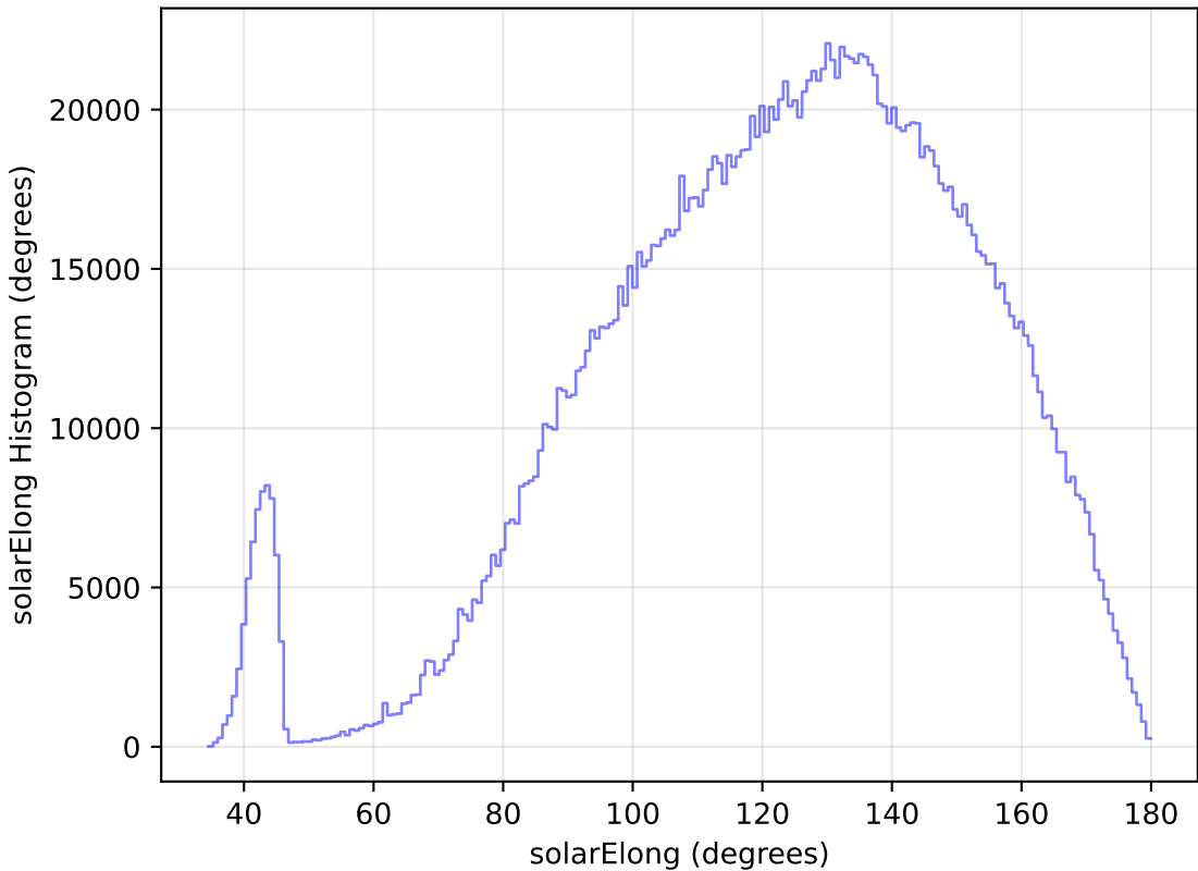
extra_ss_neo4_v3.4_10yrs WFD all bands: solarElong Histogram
