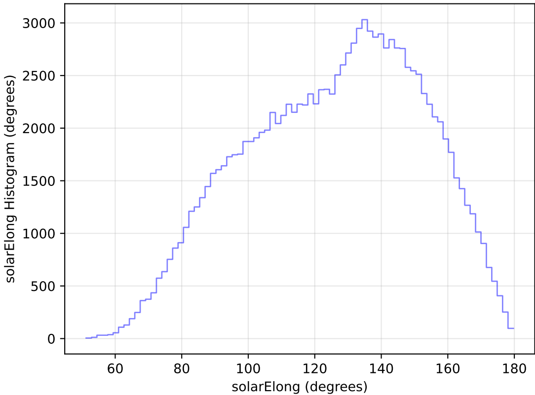
extra_ss_neo4_v3.4_10yrs All sky u band: solarElong Histogram
