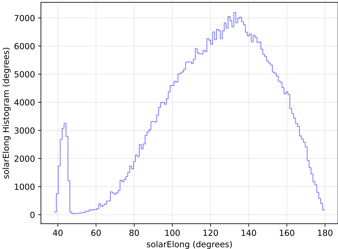
extra_ss_neo4_v3.4_10yrs All sky r band: solarElong Histogram
