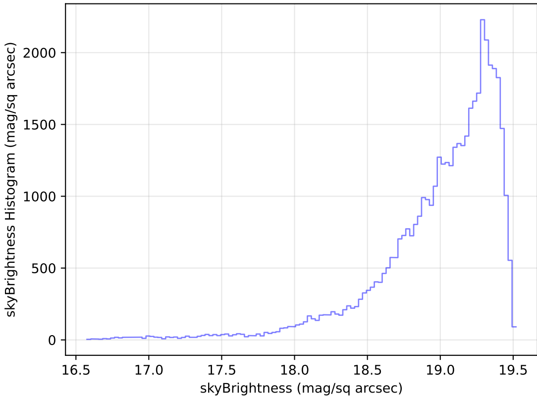
extra_ss_neo4_v3.4_10yrs Yr 1 z band: skyBrightness Histogram
