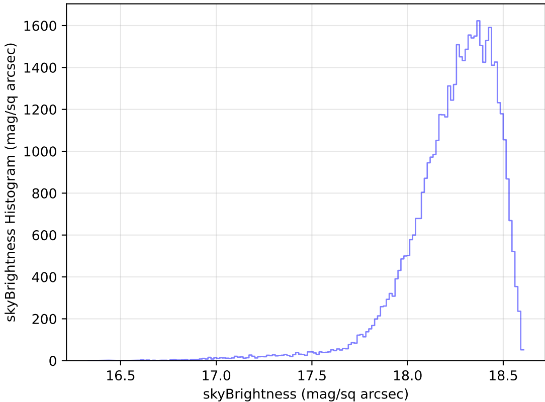
extra_ss_neo4_v3.4_10yrs Yr 1 y band: skyBrightness Histogram
