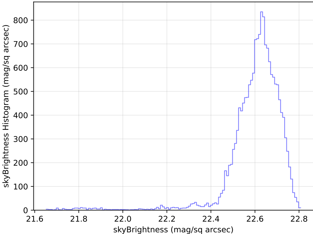
extra_ss_neo4_v3.4_10yrs Yr 1 u band: skyBrightness Histogram
