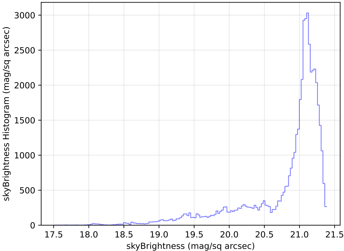
extra_ss_neo4_v3.4_10yrs Yr 1 r band: skyBrightness Histogram
