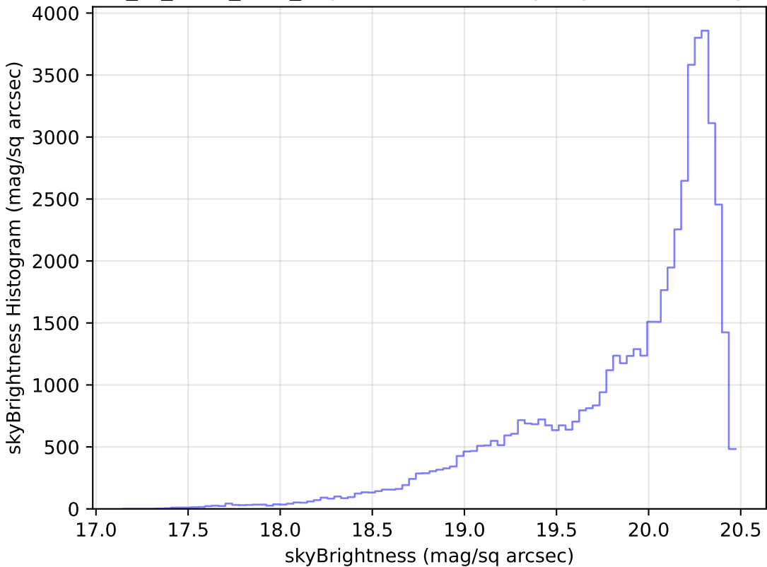
extra_ss_neo4_v3.4_10yrs Yr 1 i band: skyBrightness Histogram
