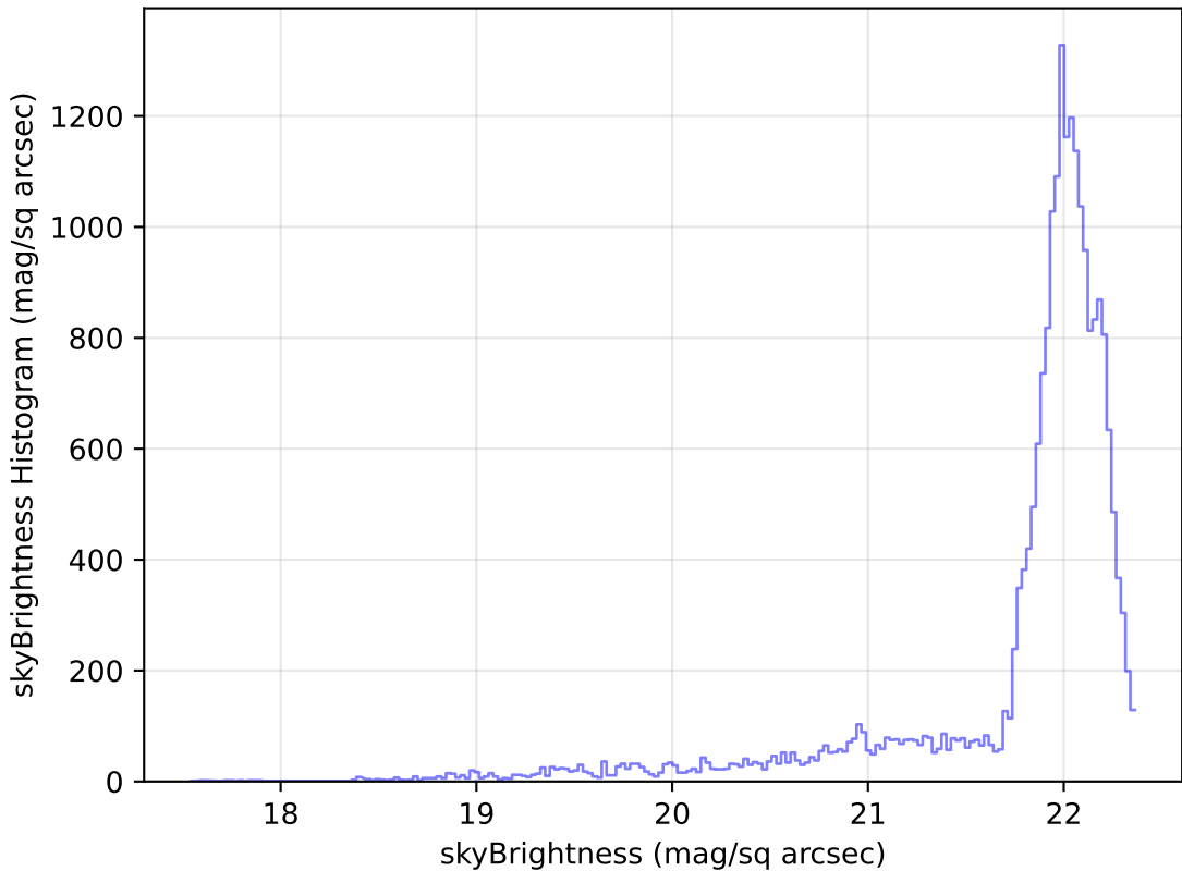
extra_ss_neo4_v3.4_10yrs Yr 1 g band: skyBrightness Histogram
