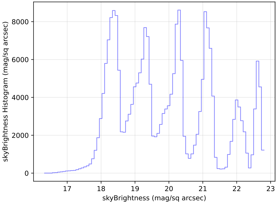
extra_ss_neo4_v3.4_10yrs Yr 1 all bands: skyBrightness Histogram
