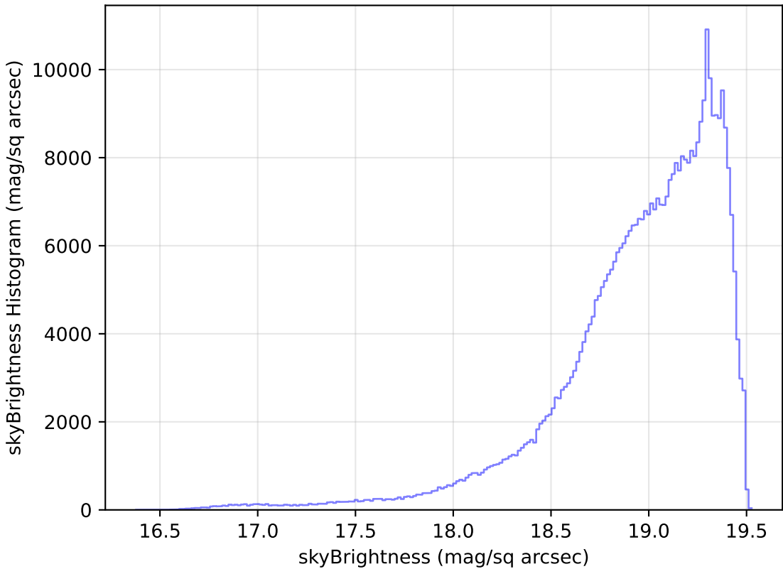
extra_ss_neo4_v3.4_10yrs WFD z band: skyBrightness Histogram
