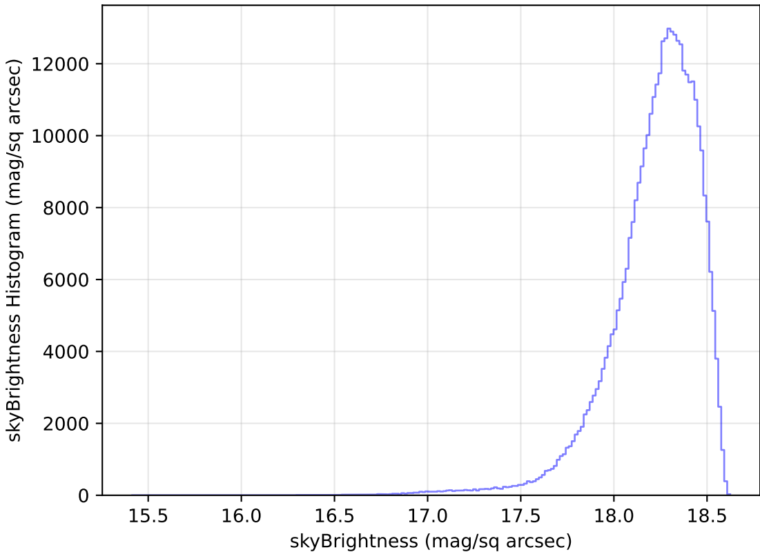
extra_ss_neo4_v3.4_10yrs WFD y band: skyBrightness Histogram
