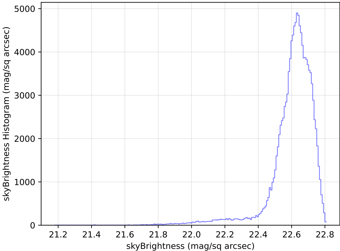
extra_ss_neo4_v3.4_10yrs WFD u band: skyBrightness Histogram
