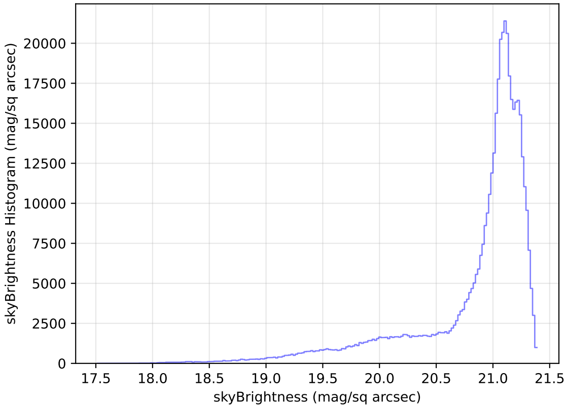
extra_ss_neo4_v3.4_10yrs WFD r band: skyBrightness Histogram
