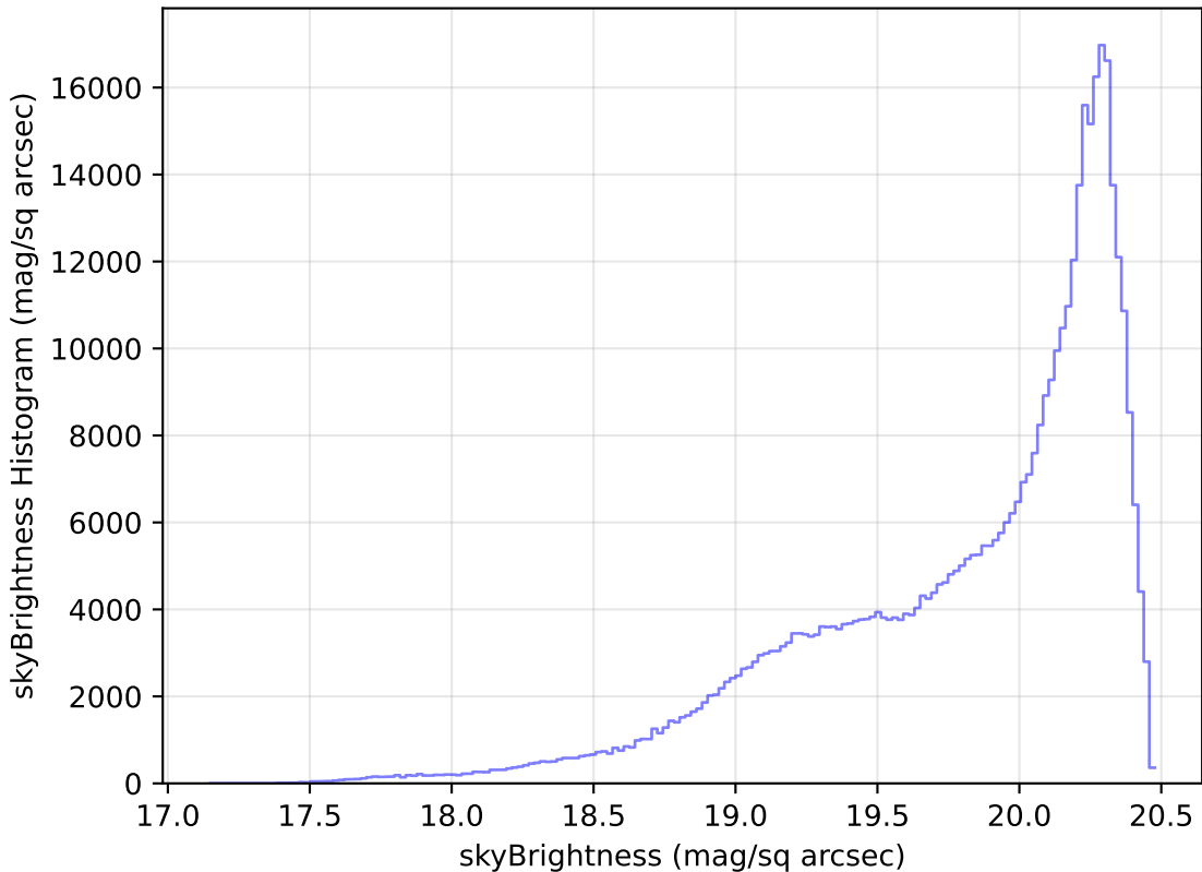
extra_ss_neo4_v3.4_10yrs WFD i band: skyBrightness Histogram
