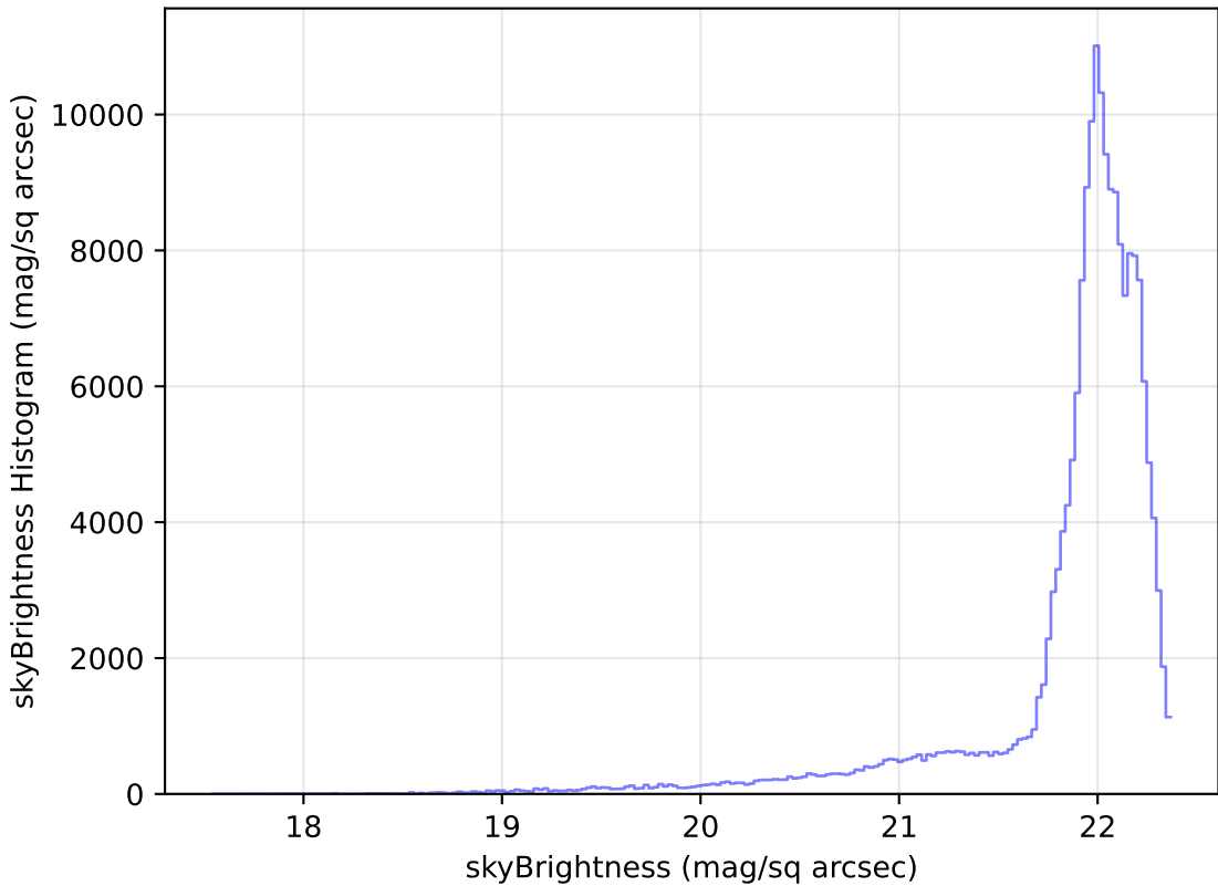
extra_ss_neo4_v3.4_10yrs WFD g band: skyBrightness Histogram
