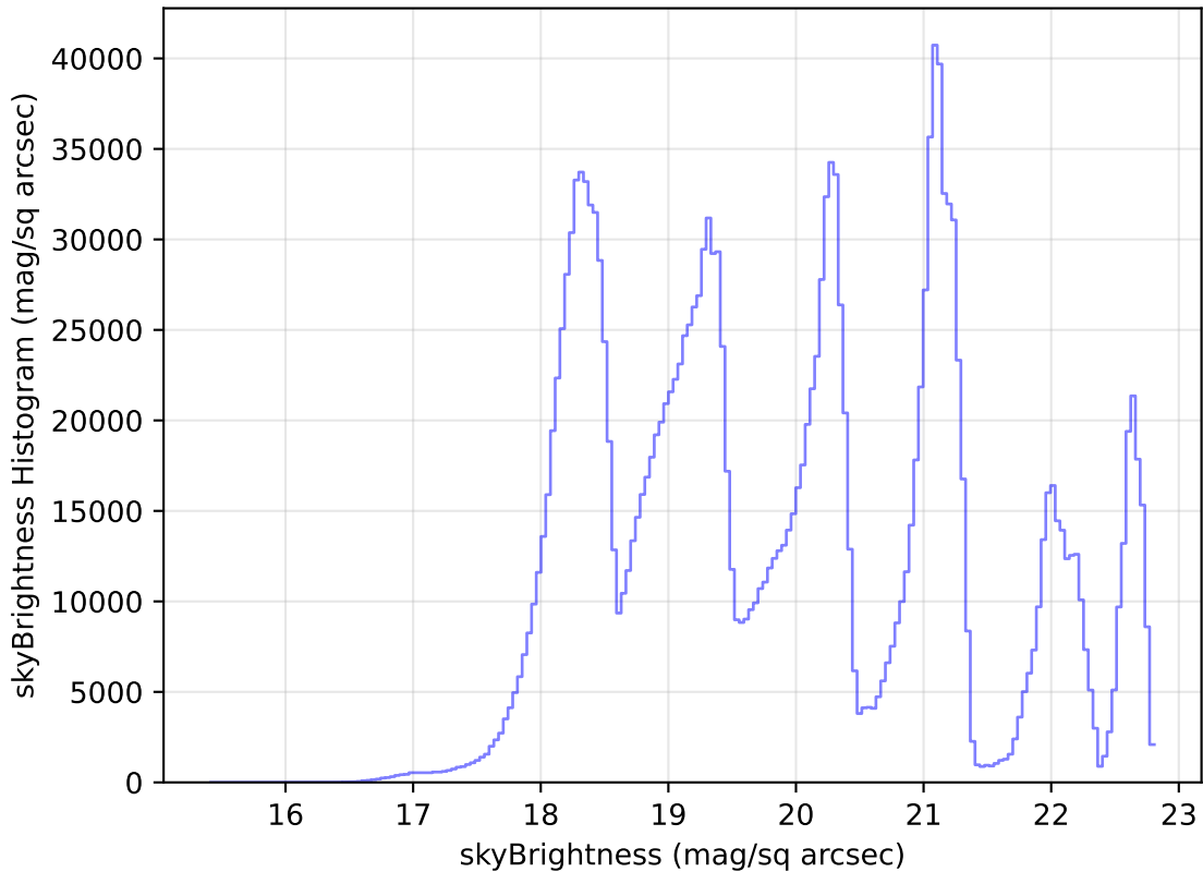
extra_ss_neo4_v3.4_10yrs WFD all bands: skyBrightness Histogram
