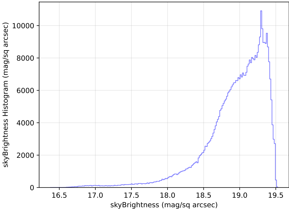
extra_ss_neo4_v3.4_10yrs All sky z band: skyBrightness Histogram
