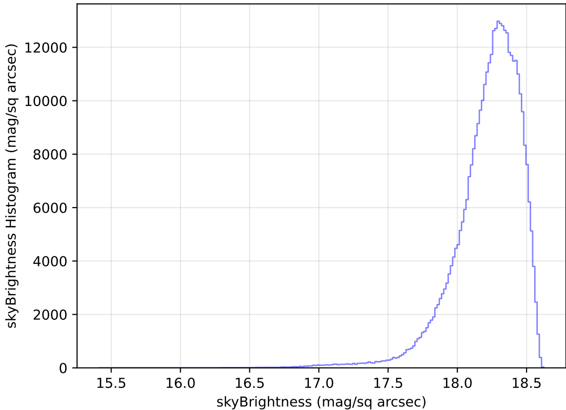
extra_ss_neo4_v3.4_10yrs All sky y band: skyBrightness Histogram
