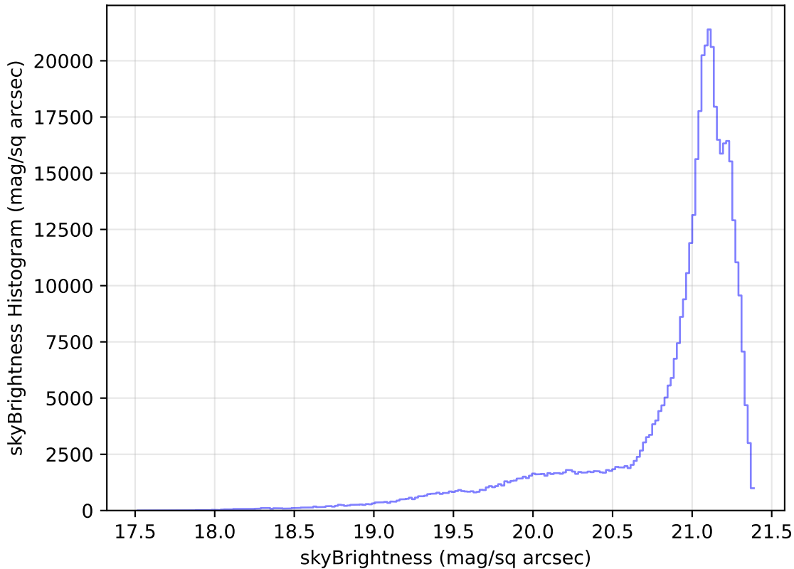
extra_ss_neo4_v3.4_10yrs All sky r band: skyBrightness Histogram
