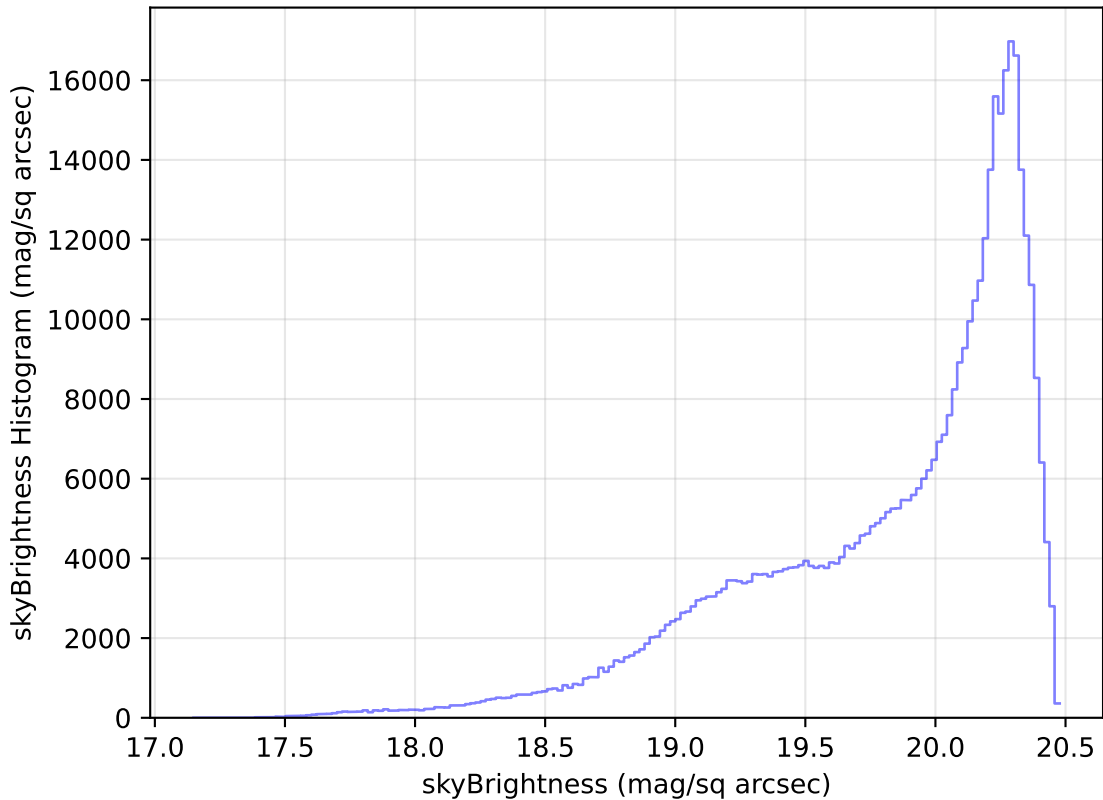
extra_ss_neo4_v3.4_10yrs All sky i band: skyBrightness Histogram
