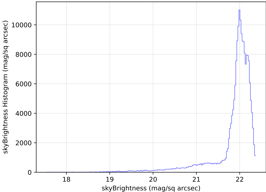
extra_ss_neo4_v3.4_10yrs All sky g band: skyBrightness Histogram
