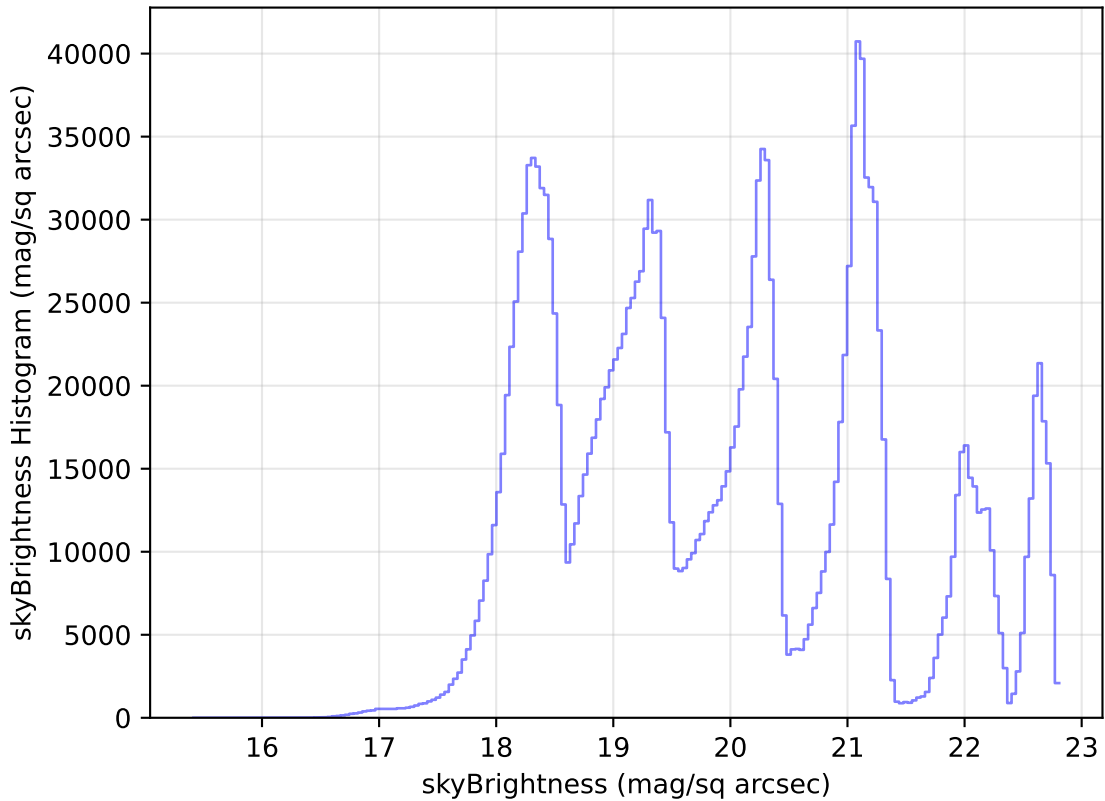
extra_ss_neo4_v3.4_10yrs All sky all bands: skyBrightness Histogram
