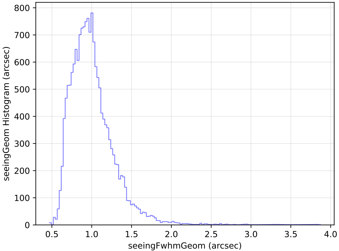
extra_ss_neo4_v3.4_10yrs Yr 1 u band: seeingGeom Histogram
