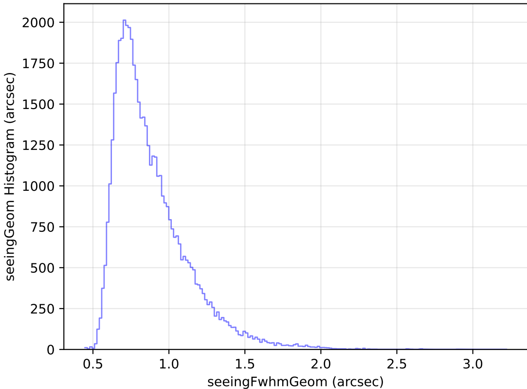
extra_ss_neo4_v3.4_10yrs Yr 1 r band: seeingGeom Histogram
